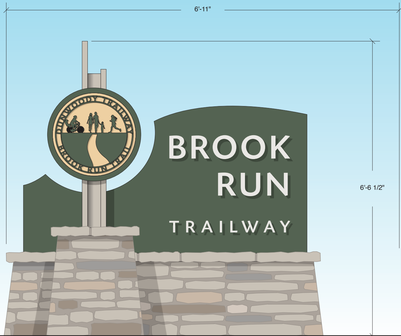
1 TRAILHEAD MARKER - FRONT ELEVATION SCALE: 3/4" = 1'-0"
