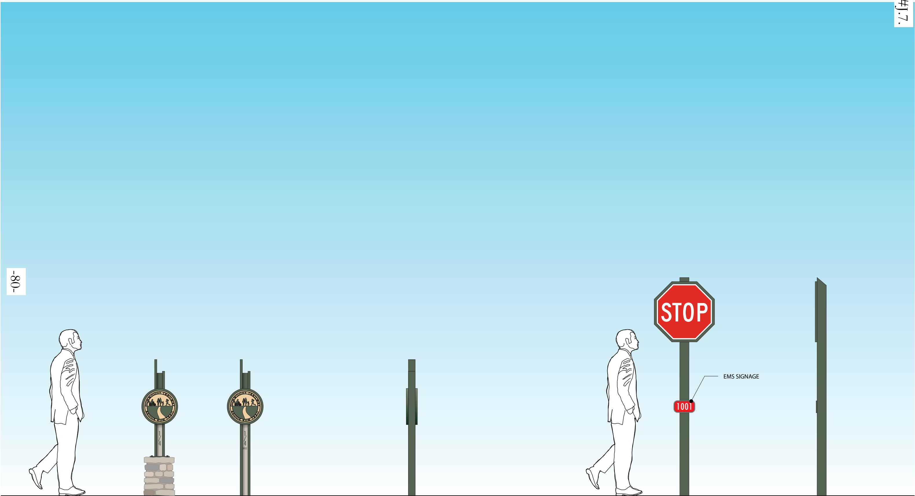
1 DISTANCE MARKER (WITH AND WITHOUT STONE BASE) - FRONT ELEVATION SCALE: 1/2" = 1'-0"
