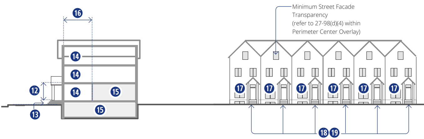
Figure 27-105-10 Townhouse Building: Floor-to-Floor Height & Use Requirements
