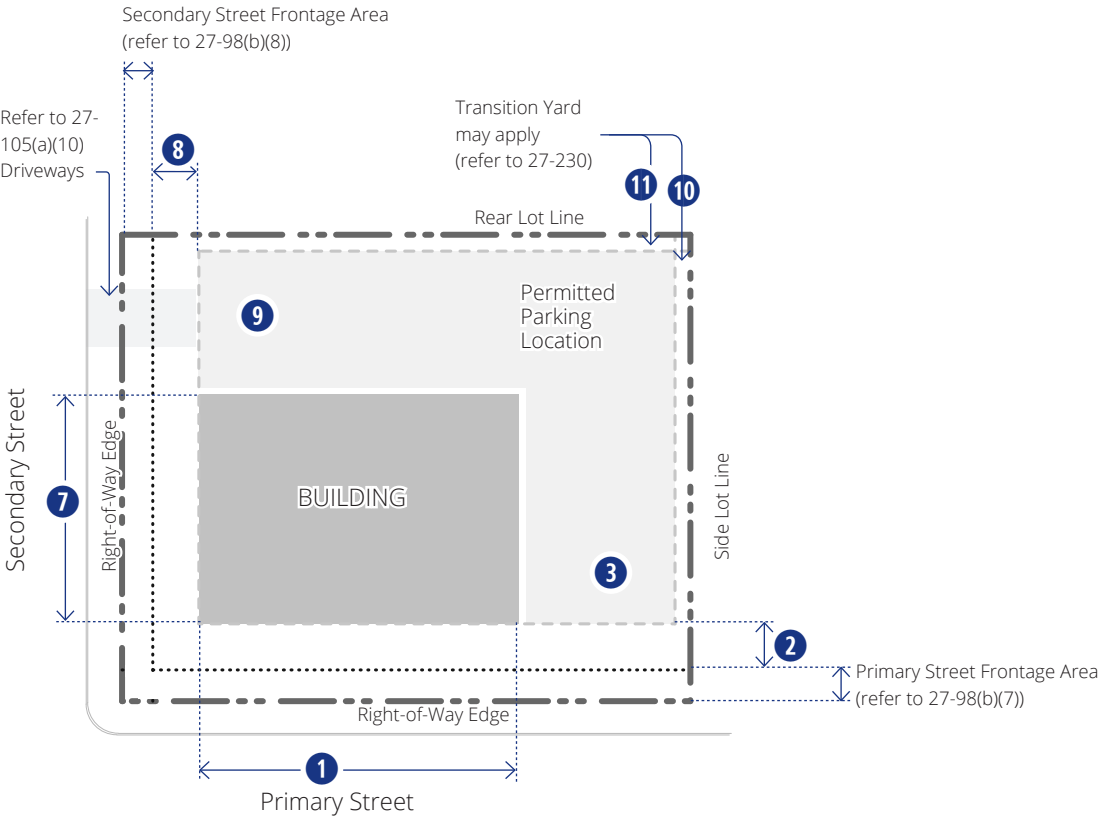
Figure 27-105-15 Civic Building: Building Siting
