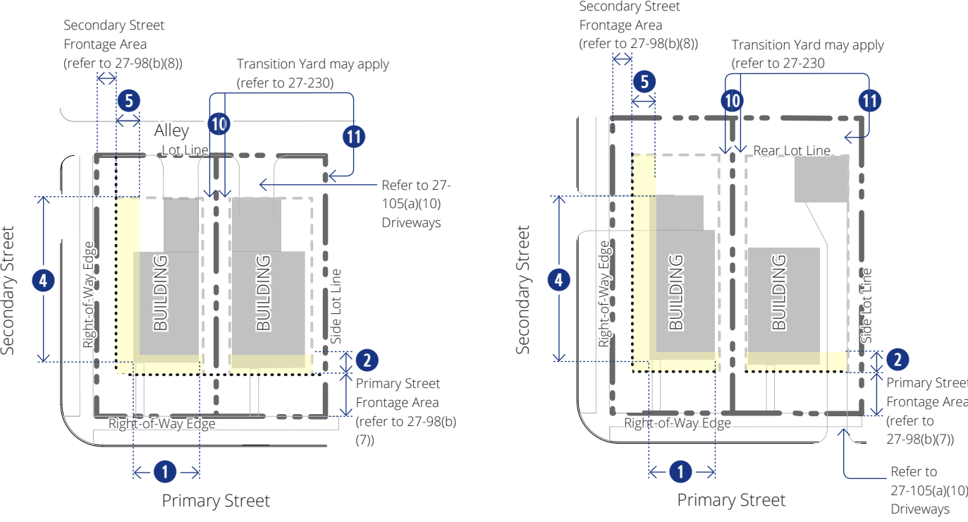
Figure 27-105-12 Detached House Building: Building Siting
