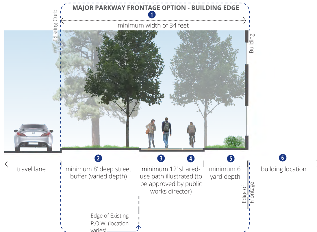
Figure 27-98-8 Major Parkway Frontage Option - Building Edge
