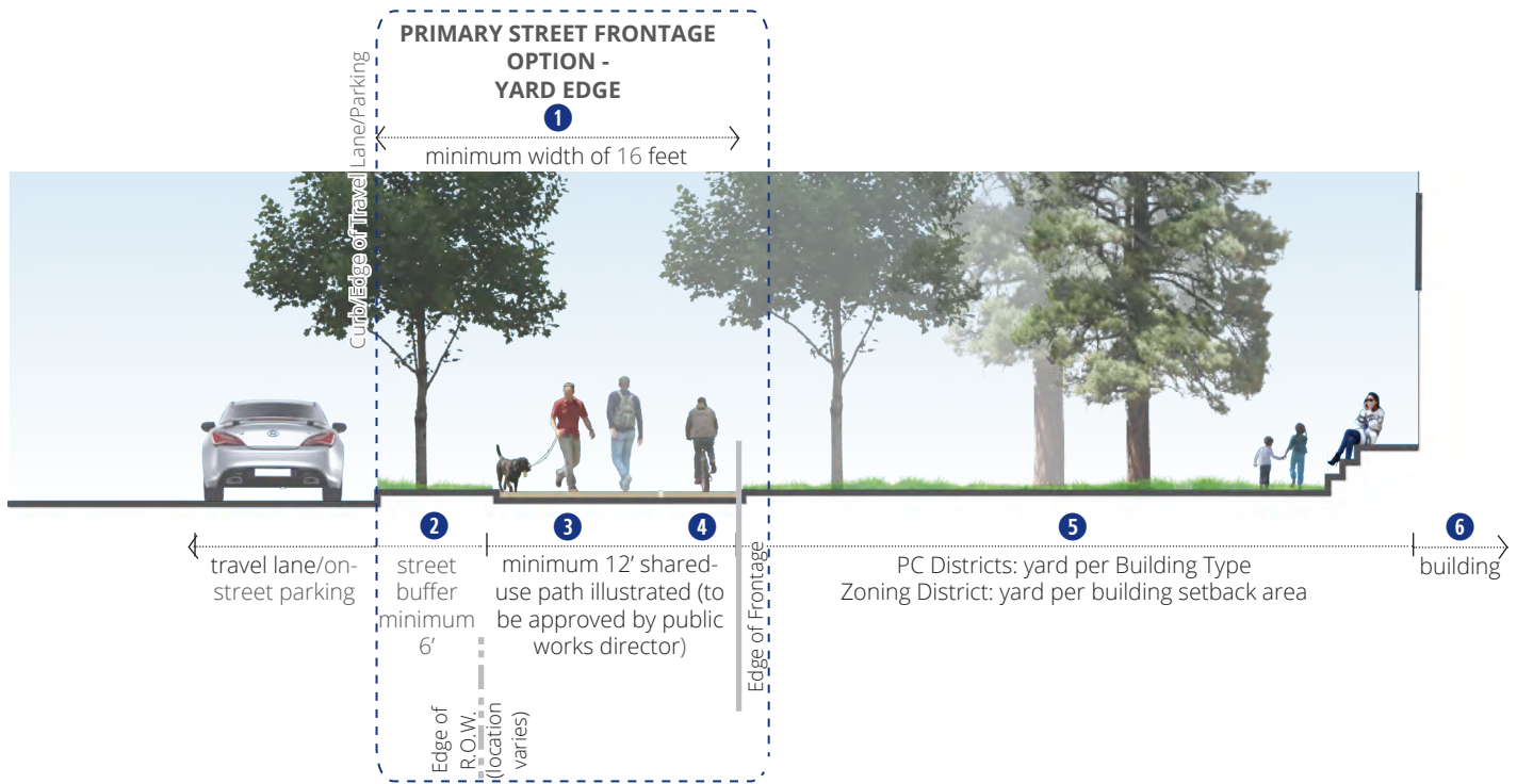
Figure 27-98-21 Primary Street Frontage Option - Yard Edge
