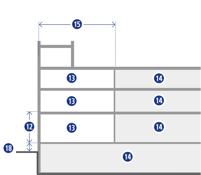
Figure 27-105-16 Civic Building: Floor-to-Floor Height & Use Requirements
