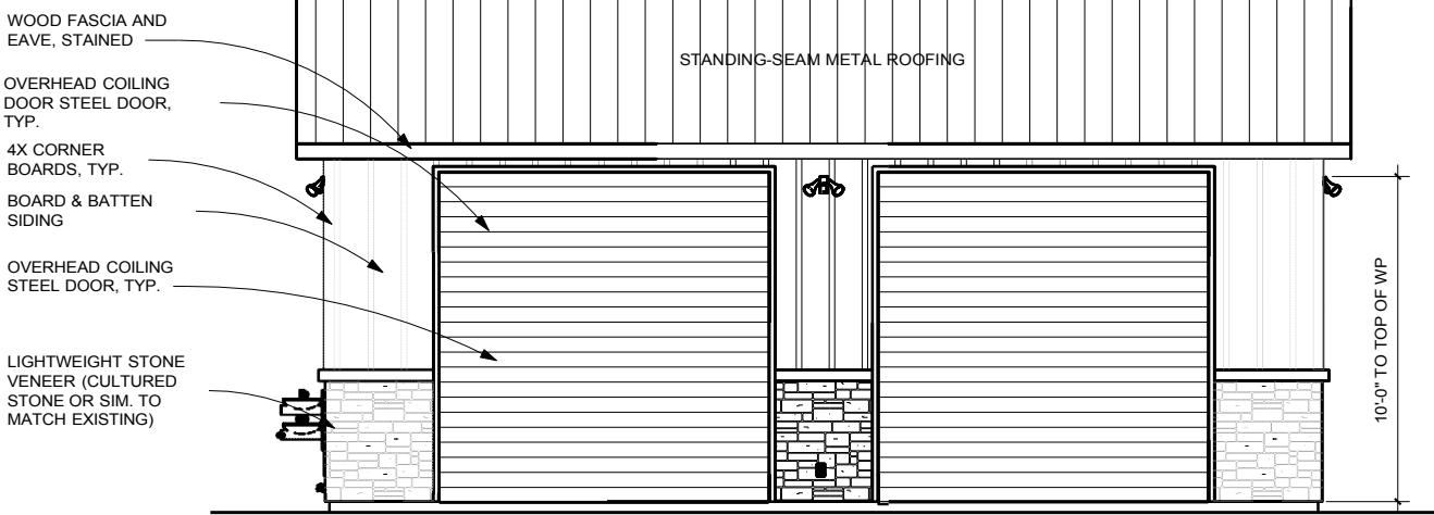
5 REAR ELEVATION A1.1 1/4" = 1'-0"
