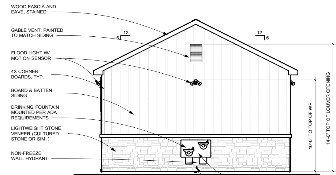
6 LEFT ELEVATION A1.1 1/4" = 1'-0"
