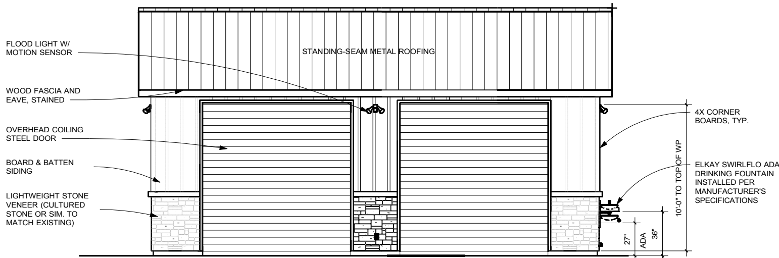
2 FRONT ELEVATION A1.1 1/4" = 1'-0"
