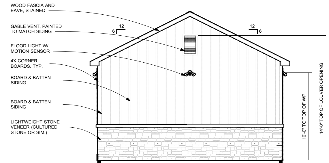
4 RIGHT ELEVATION A1.1 1/4" = 1'-0"
