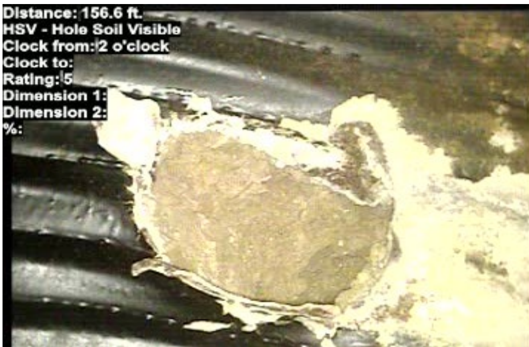
Corrosion with visible holes
