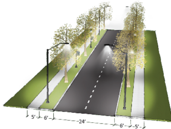
OPTION B COMBINATION OF PEDESTRIAN (TYPE P) AND STANDARD COBRA HEAD (TYPE C) FIXTURES. TREES SPACED 60' O.C.
