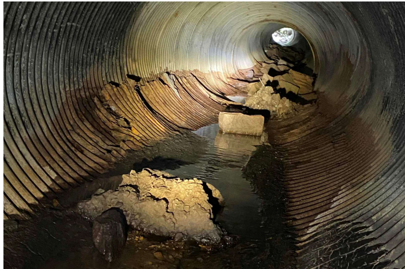
Extensive Corrosion and Large Rock Debris in 54-inch CMP
